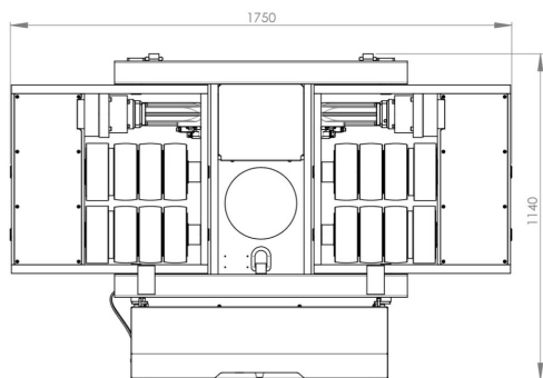
JLA-e 25/50 H | Art.No. 22 025 200-G| Draufsicht | Top view
