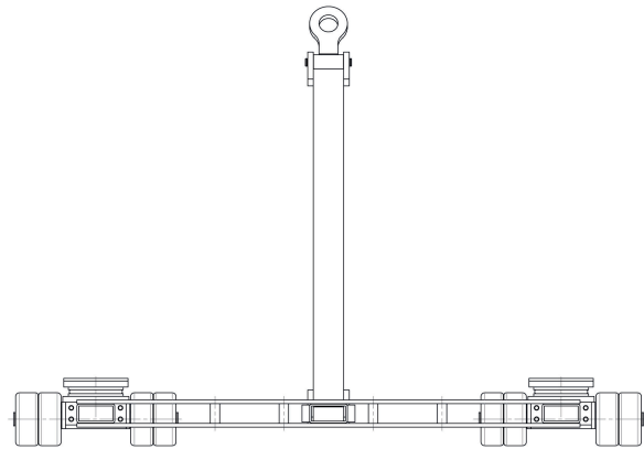
JTL 20 G | Art.No. 12 202 140-V | Frontansicht | Front view
